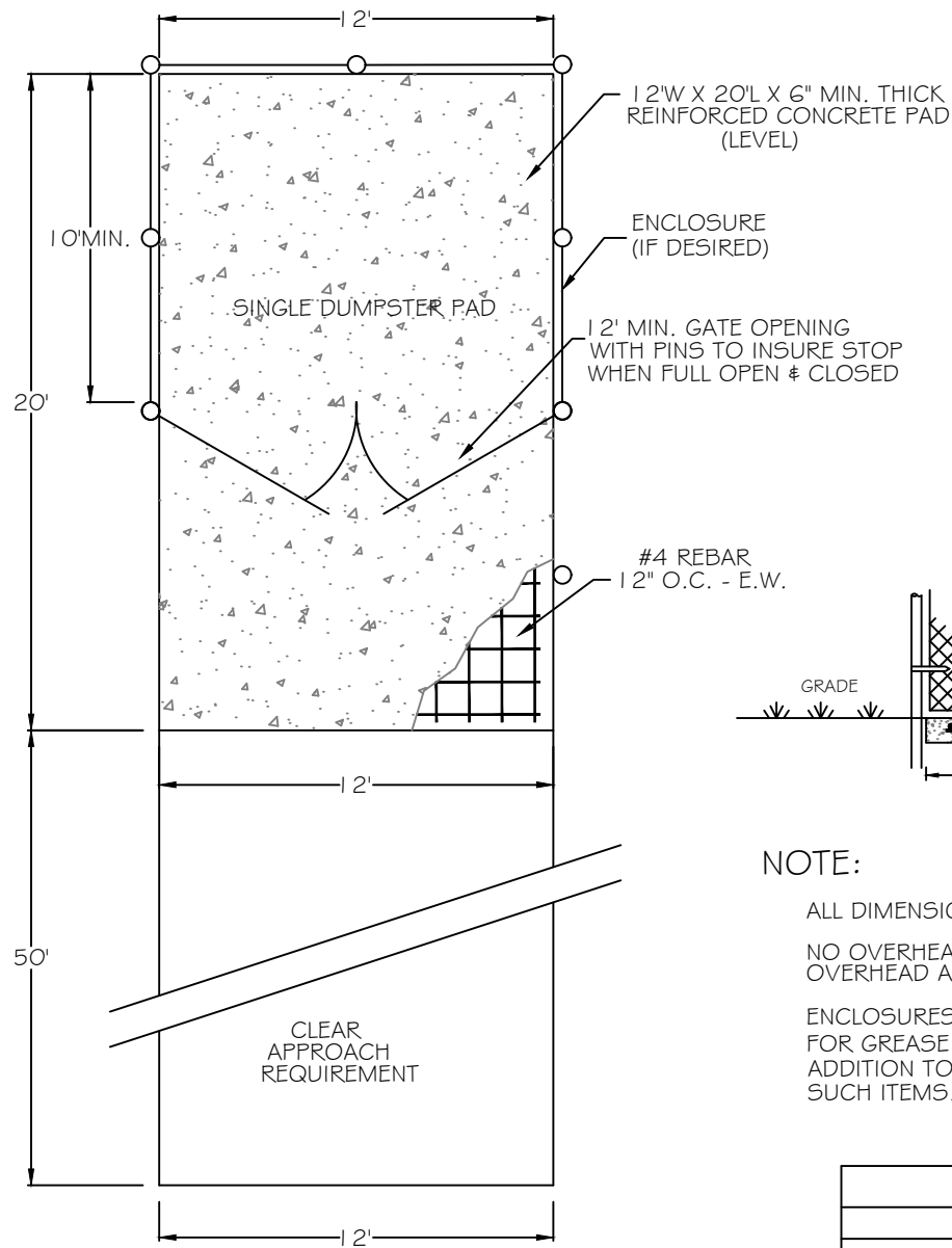
PLAN VIEW SINGLE DUMPSTER PAD
